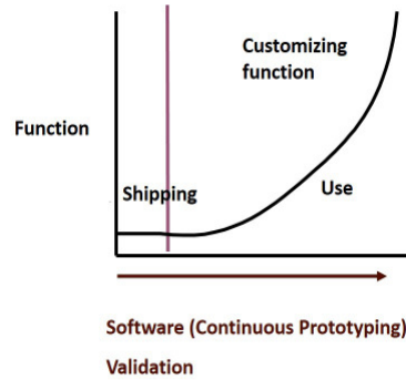
Fig. 2. Software development
