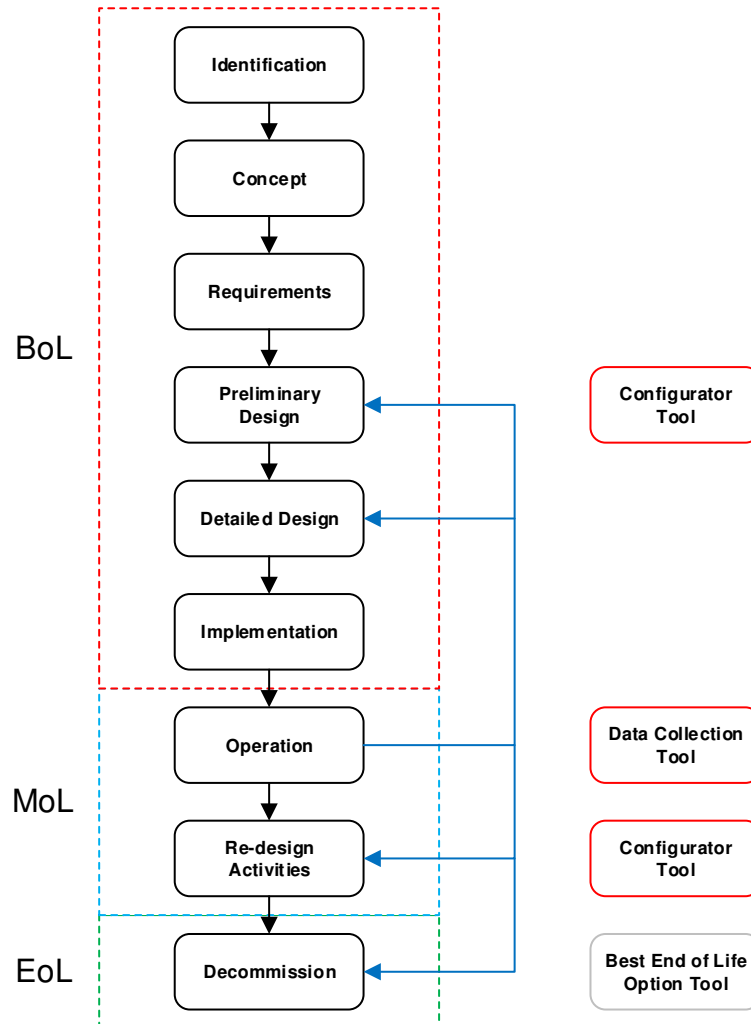
Fig. 2. Closed Loop Framework
