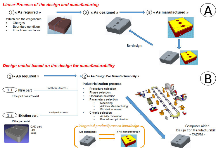
Figure 1 Design and manufacturing strategy's implemented in the product development.
