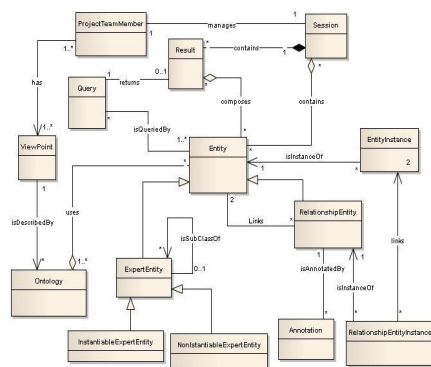
Fig. 2. The extended conceptual model of Relationship Manager
