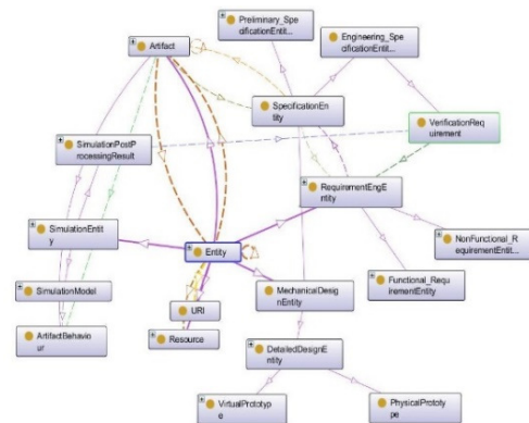
Fig. 3. Main entities of the proposed product BOL ontology
