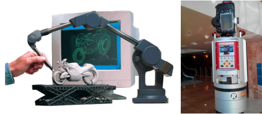
Fig. 1 3D scanning devices. Left: A contact-based MicroScribe device (photo taken from [3]). Right: The Riegl VZ-400 terrestrial laser scanner.
