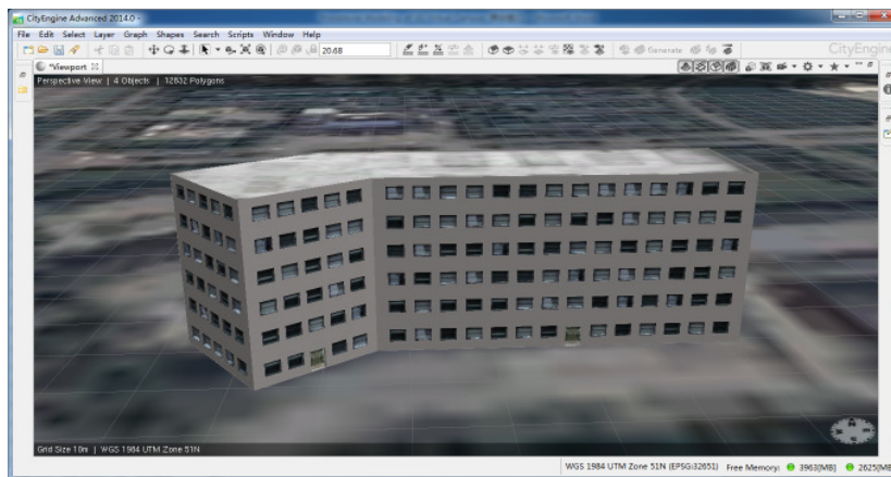
Fig. 6. 3D model of building created in CityEngine based on CGA rules.
