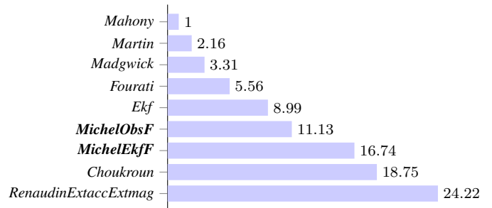
Fig. 9. Relative performance in terms of CPU cost (lower is better).
