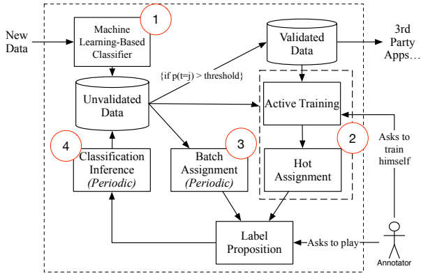
Figure 1: Framework Architecture.
