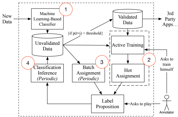
Figure 1: Framework Architecture.
