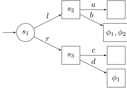
Figure 7: Example showing that AG \not\equiv AA . Player 1 controls circle states and player 2 square states.
