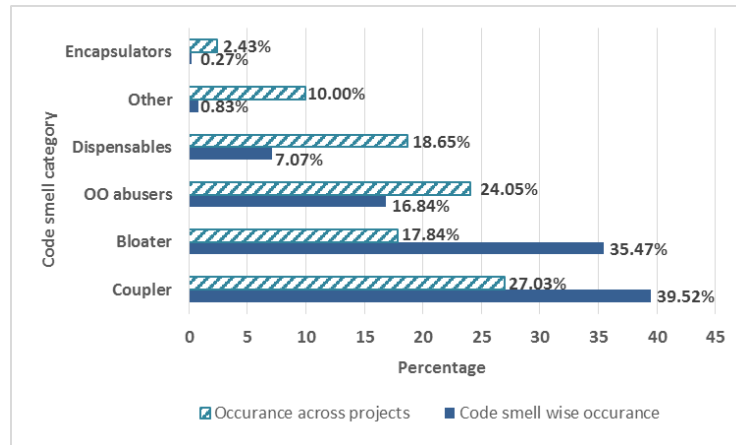
Fig. 1. Percentage occurrence of code smell categories
