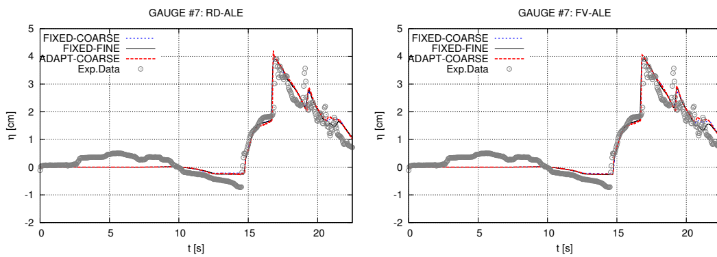
Figure 21: Okushiri experiment: total water height \eta signal registered at the gauges g7. Left: RD-ALE scheme. Right: FV-ALE scheme.
