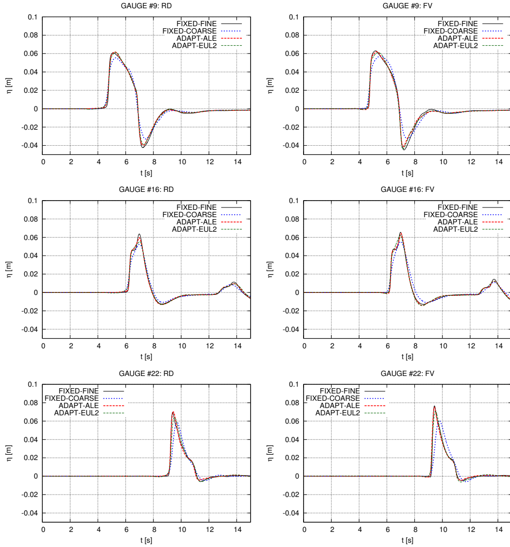
Figure 18: Conical Island: comparison between adaptive algorithms and fixed grid computations. Total water height \eta signal registered at the gauges g9, g16, g22. Left: RD scheme. Right: FV scheme.
