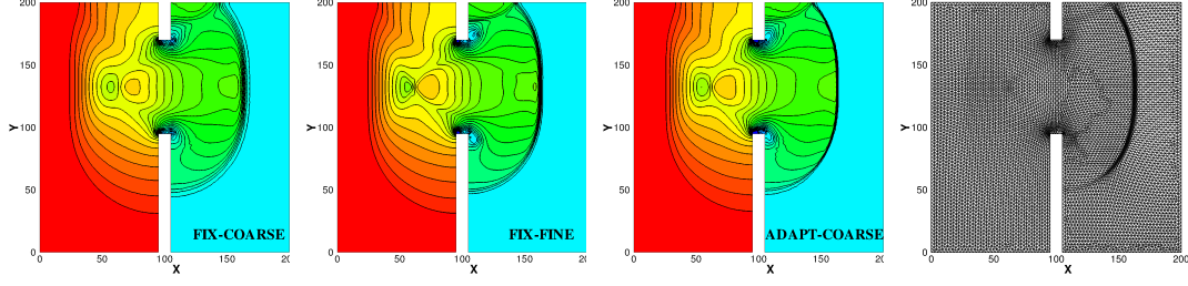
Figure 5: Asymmetric dam-break computed with RD scheme. 30 equispaced contour lines for h and adapted mesh.
