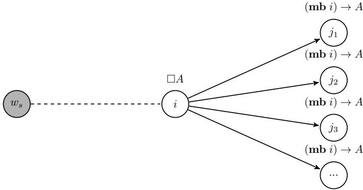
FIGURE 3 Possible Worlds Hierarchy of \Box A
