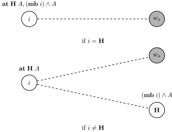
FIGURE 4 Possible Worlds Hierarchy of at H A
