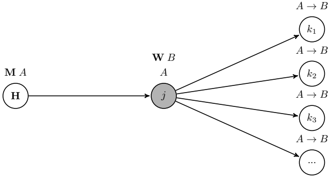
FIGURE 3 Possible Worlds Hierarchy of Example (14)
