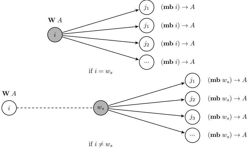
FIGURE 6 Possible Worlds Hierarchy of \llbracket \textit{would} \rrbracket_{M-TTDLA}
