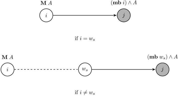
FIGURE 5 Possible Worlds Hierarchy of \llbracket \text{might} \rrbracket_{M-TTDLA}
