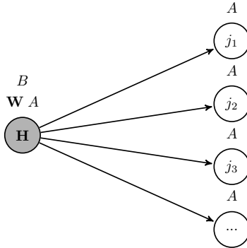
FIGURE 2 Possible Worlds Hierarchy of Example (13-b)
