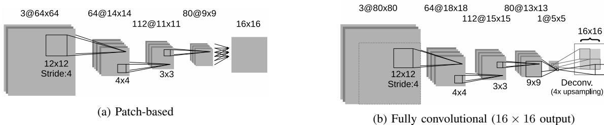
Fig. 1: Convolutional neural network architectures (e.g., “64@14 × 14” means 64 feature maps of size 14 × 14).
