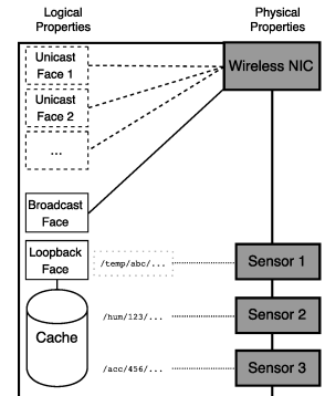
Figure 2. IoT device.
