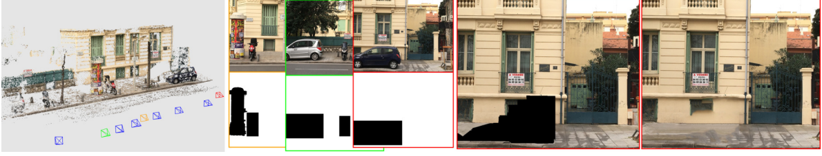
Figure 1. (a) 3D reconstruction from multi-view input image dataset (b) Input images above, input masks below (c) Result of reprojection and mincut, remaining black pixels will be filled through patch-based inpainting (d) Inpainted result.
