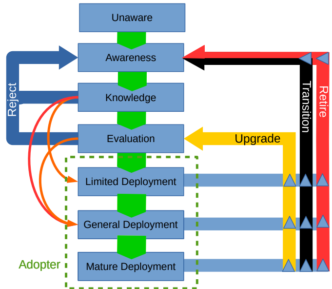
Fig. 2: proposed OSS staged adoption model
