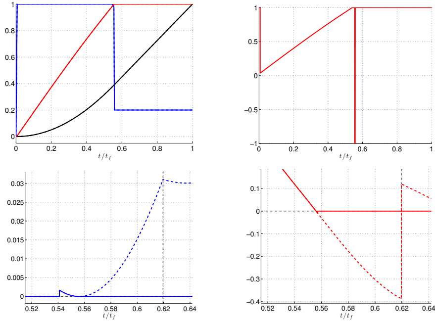
FIGURE 13. Trajectories \gamma_+ \gamma_{c_1} \gamma_+ \gamma_- \gamma_+^{c_3} and \gamma_+ \gamma_{c_1} \gamma_+ \gamma_- \gamma_{c_3} , with u_{c_3}(\cdot) = +1 . The BC-extremal \gamma_+ \gamma_{c_1} \gamma_+ \gamma_- \gamma_+^{c_3} at v_{\max} = v_{\max}^{\gamma_{c_3}} from h_3 is represented by dashed lines while the one \gamma_+ \gamma_{c_1} \gamma_+ \gamma_- \gamma_{c_3} from h_4 is represented by solid lines. (Top-Left) The state trajectories. (Top-Right) The control. (Bottom-Left) Zoom on the component p_1(\cdot) . (Bottom-Right) Zoom on the component p_3(\cdot) . About the trajectory \gamma_+ \gamma_{c_1} \gamma_+ \gamma_- \gamma_{c_3} with u_{c_3}(\cdot) = +1 , the components p_1(\cdot) and p_3(\cdot) are identically zero along \gamma_{c_3} since this extremal is a limit case from h_4 for which for each solution, the functions \Phi and \dot{\Phi} are zero along \gamma_{c_3} . Note that the sine wave shapes of the trajectory at Figure 7 have changed into square wave shapes.
