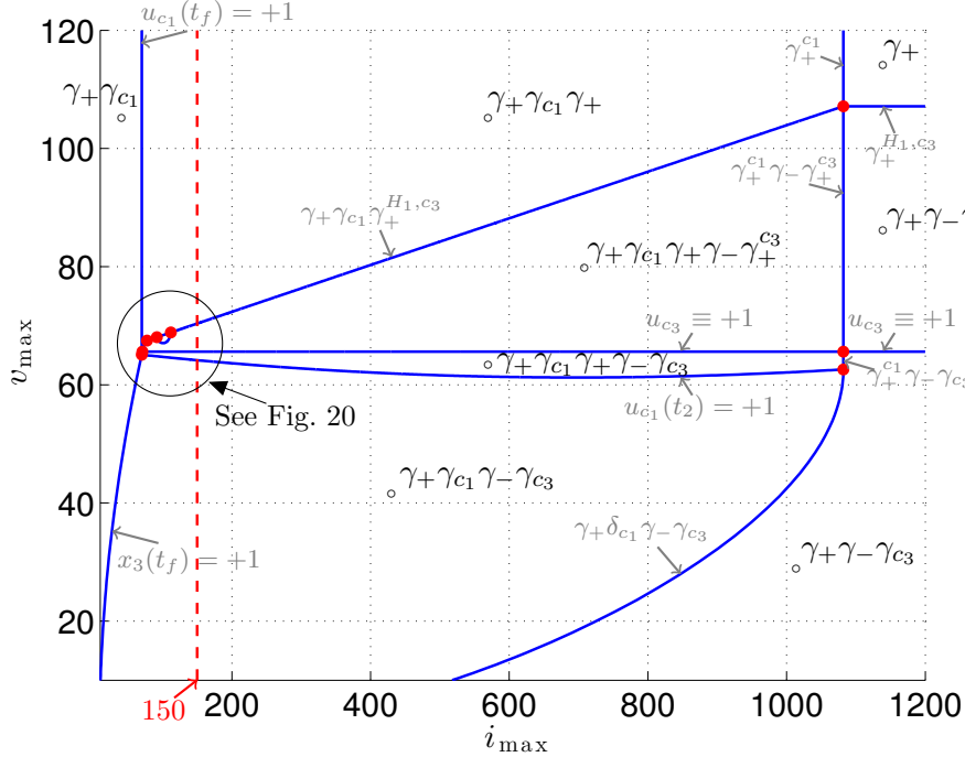
FIGURE 19. Synthesis with respect to i_{\max} and v_{\max} . The structures are displayed on the graph. The sequence labeled \gamma_+\delta_{c_1}\gamma_+ means that there is a contact point with the constraint set C_1 at the switching time between \gamma_+ and \gamma_+ .
