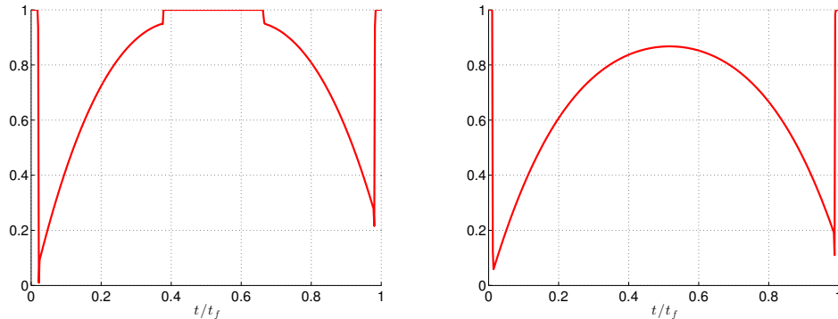
FIGURE 21. Problem ( P_{e\min} ). Optimal control for problem ( P_{e\min} ) for t_f = 1.25 T_{\min} (left) and t_f = 1.50 T_{\min} (right), with T_{\min} \approx 5.6156 , \alpha_f = 100 , i_{\max} = 1100 and v_{\max} = 110 . The structure is \gamma_+ \gamma_s \gamma_+ \gamma_s \gamma_+ for t_f = 1.25 T_{\min} and \gamma_+ \gamma_s \gamma_+ for t_f = 1.50 T_{\min} . The solutions have been computed with the Bocop [6] software.
