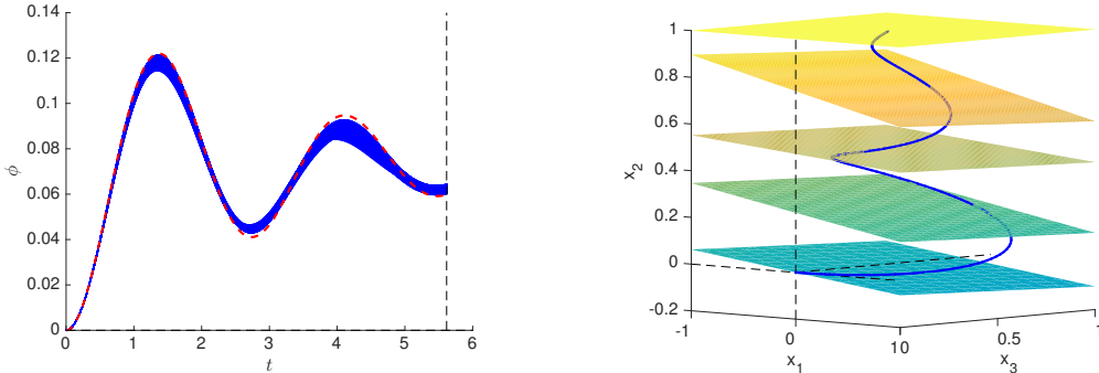
FIGURE 3. (Left) The blue plain lines represent the switching functions \phi(t) = H_1(z(t, z_f)) , t \in [0, \bar{t}_f] , for a set of points z_f := (x_f, p_f) with x_f \in M_f , p_f = (0, 1, 0) , where M_f is sampled using a fine grid, and where z(\cdot, z_f) is the solution of H_+ starting from z_f computed with backward integration. The red dashed line is the switching function when the dynamics eq. (2) is linear, i.e. a_6 = 0 . (Right) The evolution of M_f at times 0, 0.25 \bar{t}_f , 0.5 \bar{t}_f , 0.75 \bar{t}_f and \bar{t}_f , by backward integration. The blue curve is the optimal \gamma_+ trajectory.
