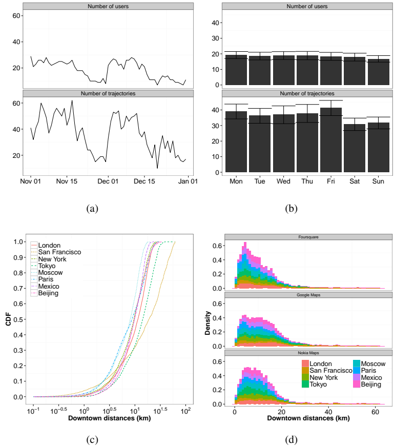
Figure 2: (Better seen in colors) (a) Number of users and trajectories per day in Beijing. (b) Number of trajectories per day grouped per day of the week in Beijing. (c) CDF of the distance from points of interest to the downtown using all sources. (d) Distance from points of interest to the downtown grouped by source.
