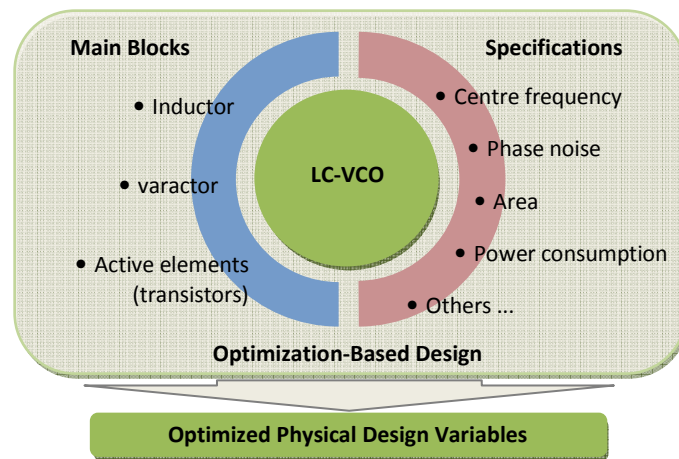
Fig. 1. LC-VCO design architecture.
