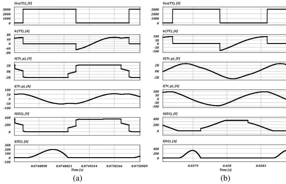
Fig. 4. Main simulation waveforms of LLC (a) and LCC (b) converters ( U_{in}=3000V , P_{out}=30kW ).
