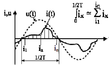
Fig. 7. Half period calculations for symmetrical non-sinusoidal current consumption.
