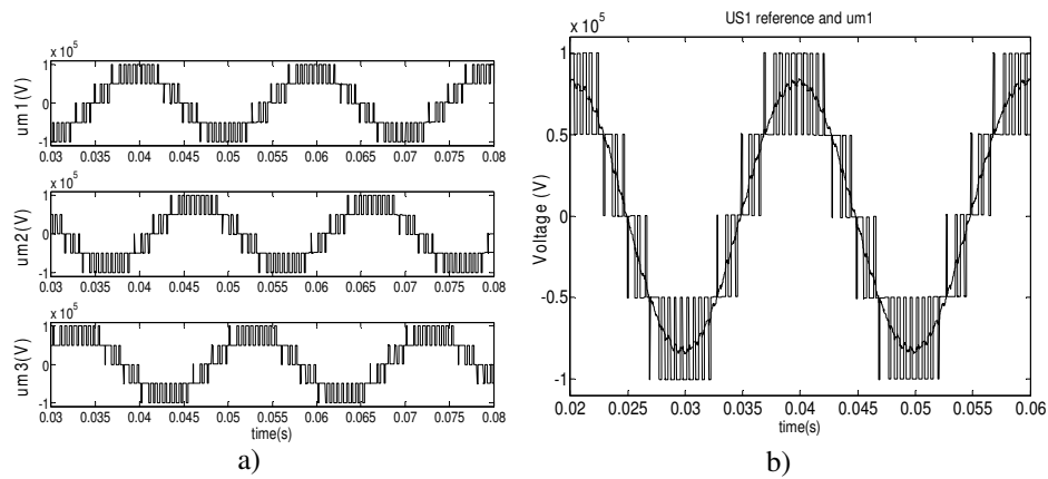
Fig. 12. Simulation results a) Three-phase ac output voltages b) U_{slref} and um1
