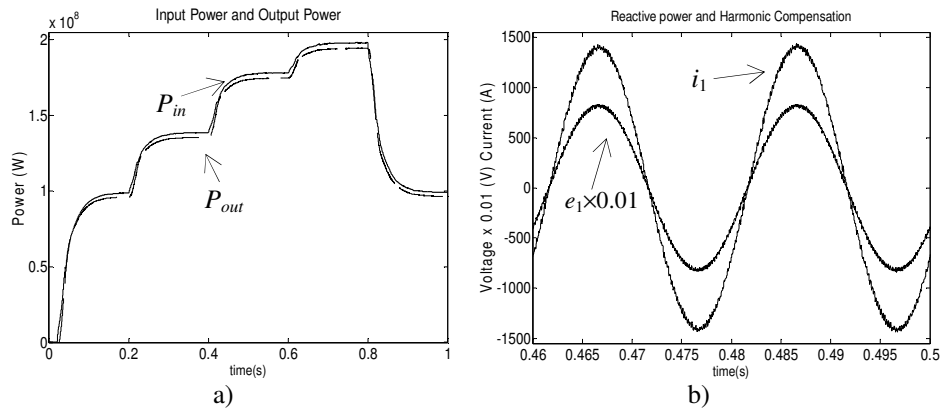
Fig. 11. Simulation results a) Output and input powers b) Current and voltage \times 0.01 in phase 1
