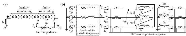
Fig. 1. (a) Equivalent circuit for a winding fault; (b) diagram of the test system.
