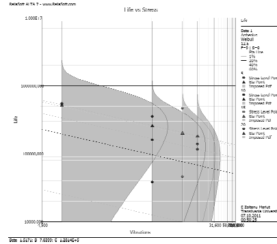
Fig. 7. Life vs. Stress profile S3, with the four vibration stress level points (5 Hz, 10 Hz, 15 Hz, 20 Hz) and the duty rating stress level 12.5 Hz.
