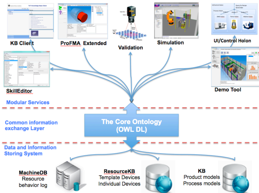
Fig. 1. Modular ICT architecture for HMS
