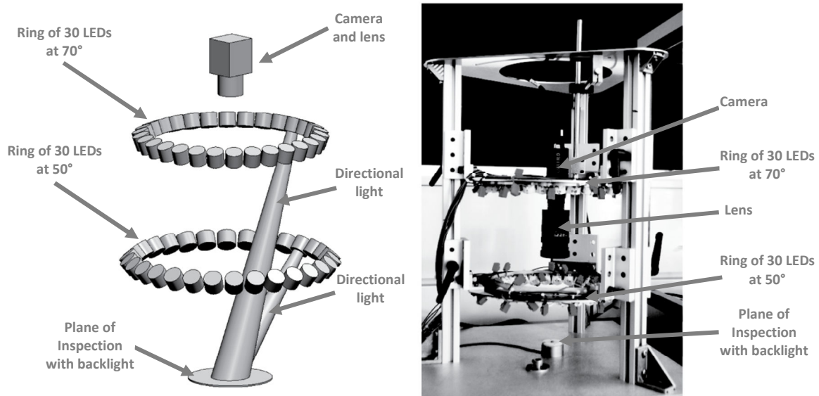
Figure 6. Acquisition setup for the inspection of the ballbearings. The axis of the camera is perpendicular to the plane of inspection. The setup allows the use of different illuminations: backlight, ringlight and directional illuminations at elevations of 50° and 70°.
