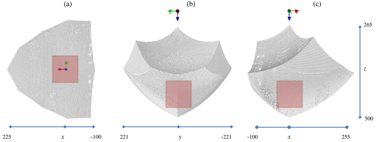
Fig. 5. The reachable workspace of the micro-CMM. (a) top view; (b) front view; (c) side view.
