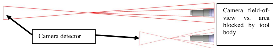
Fig 5. Pin-hole model illustrates how bringing camera closer increases the portion of camera field-of-view blocked by tool body
