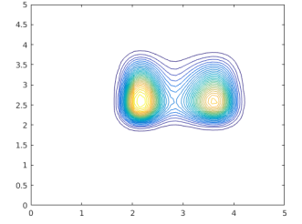
support of \nu for p = 2
