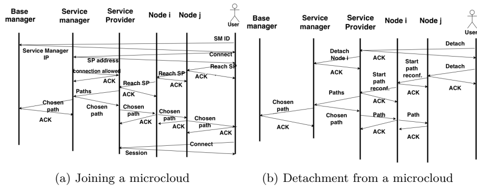
Fig. 2: Protocol description
