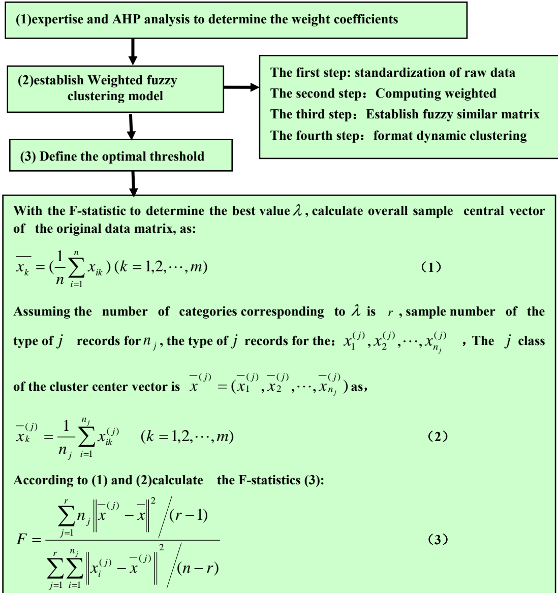
Figure 2 flow chart of the weighted fuzzy clustering
