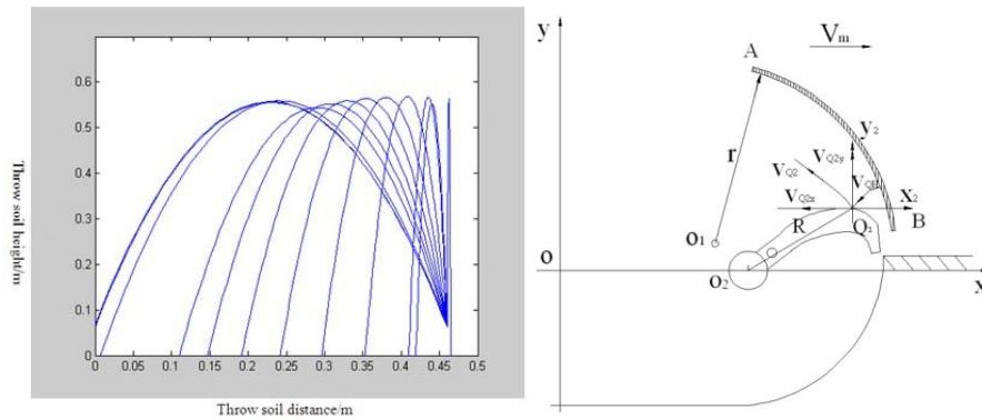
Fig. 5. Horizontal position soil distribution curve and spin plow knife position
