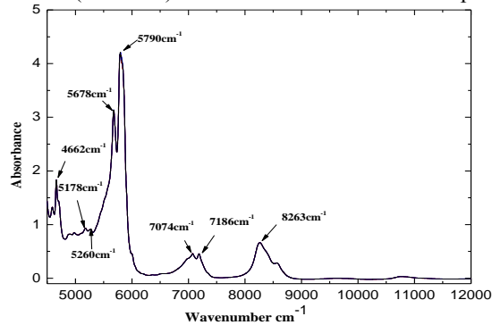
Fig.1: FT-NIR spectra in the 12,000~4,500cm -1 region of sesame oil with adulteration
