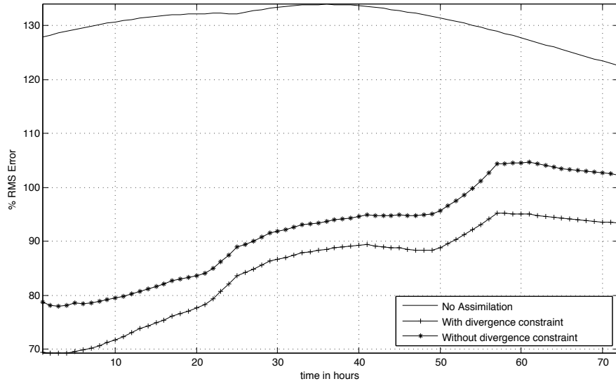
Figure 7: The effect of divergence constraint. The curve in -*- is obtained without the divergence constraint ( \alpha_2 = 0 in Eq. 9) whereas the one in -+- is obtained by adding the divergence constraint. An improvement of about 10% in the error is observed in this coastal setting. Here T_w = 24 h, \Delta t = 6 h, \sigma = 6 h, and N_f = 14 .
