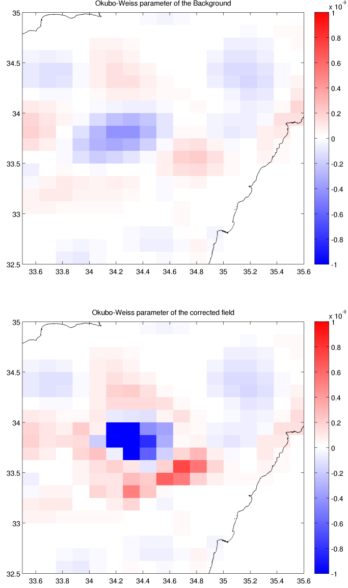
Figure 14: Okubo-Weiss parameter calculated on background field (upper panel) and corrected field (lower panel). The negativity of this parameter characterizes eddies, and the absolute value corresponds to the intensity of the eddy. It can be noticed that eddy is smaller in size and more intense after the correction process.
