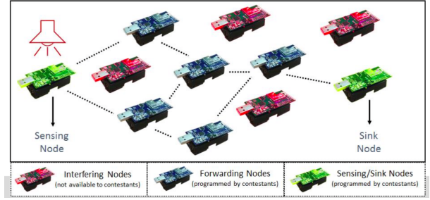
Fig. 6: Deployment scenario
