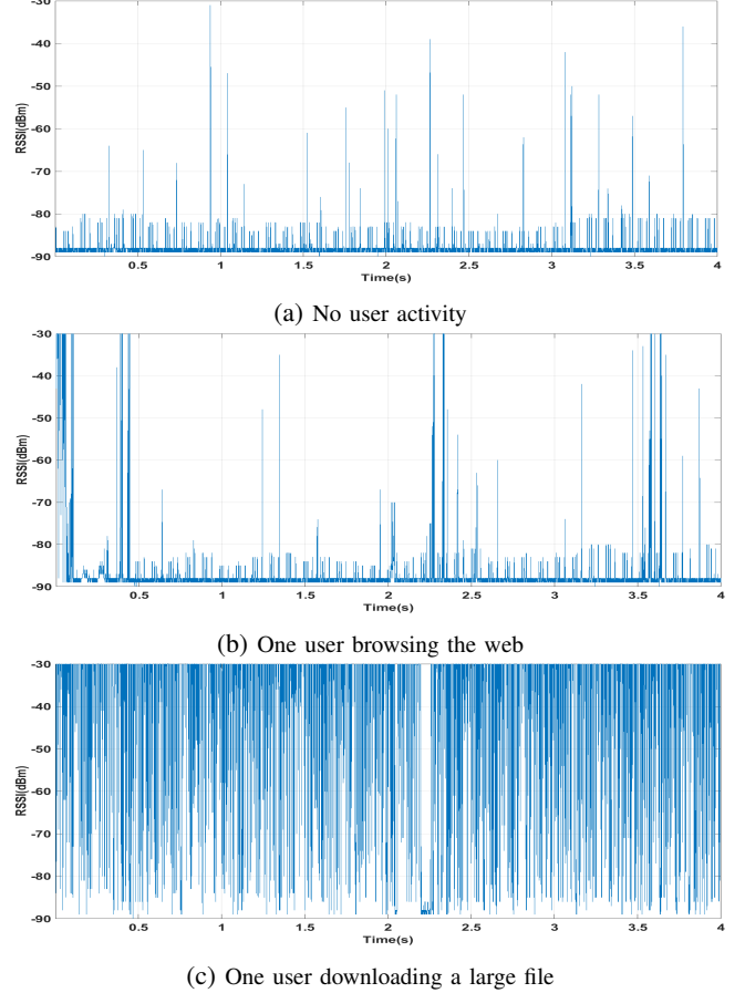
Fig. 3: Spectrum measurements
