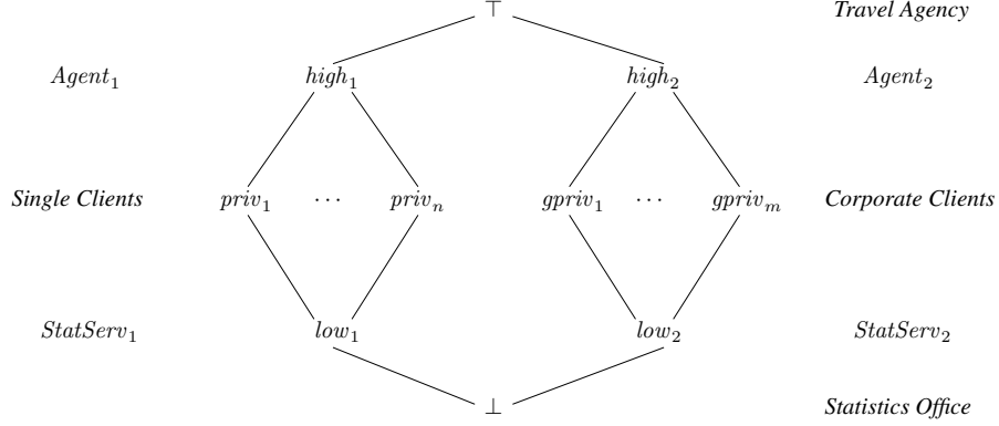
Fig. 3. Lattice of security levels for the Travel Agency example of § 4.
