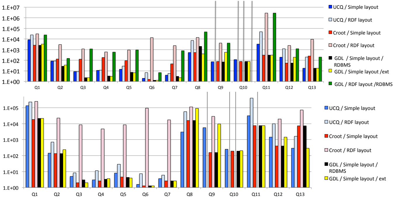
Figure 3: Evaluation time (ms) on DB2 and LUBM 2 15M (top) and 100M (bottom).
