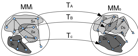
Fig. 2 Localized transformations
