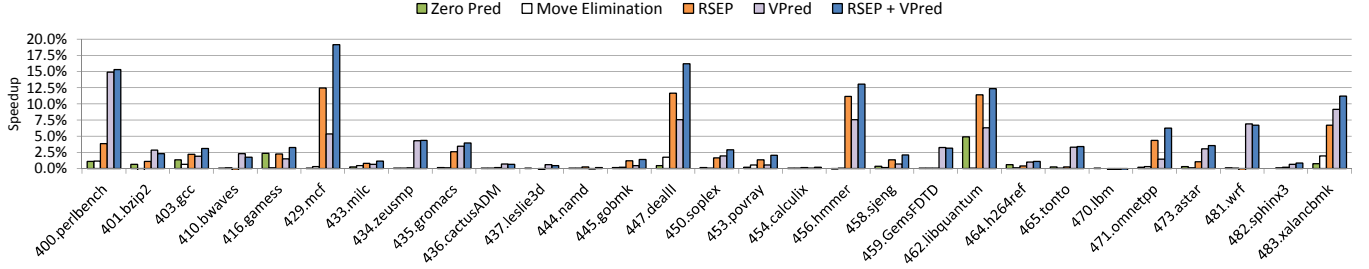
Fig. 4: Speedup over baseline using different performance-optimizing mechanisms.
