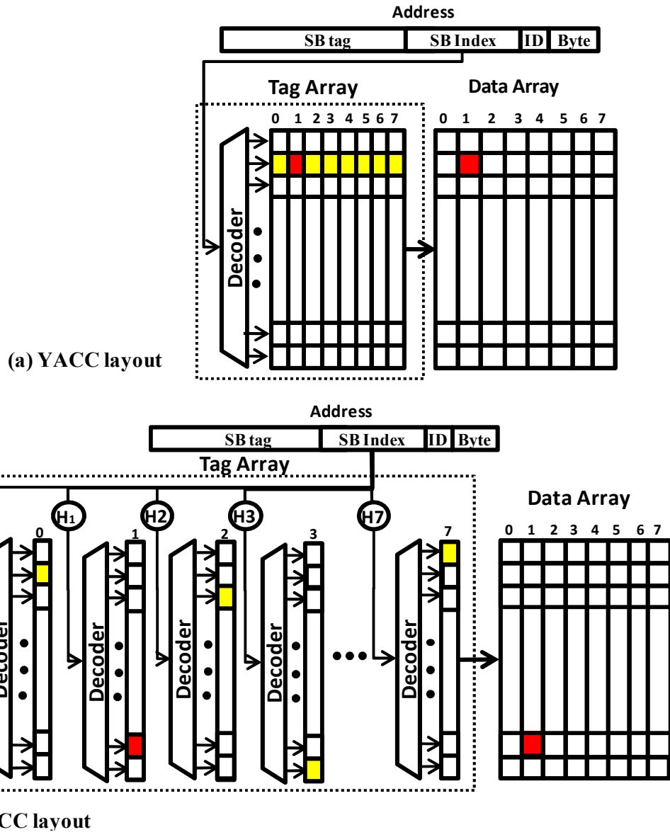
Fig. 4. Cache physical layout with YACC (a), and SCC (b)
