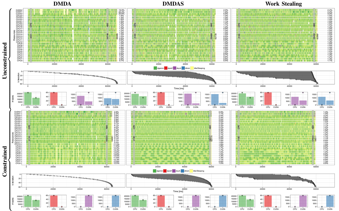
Fig. 4: The execution representation of three schedulers (DMDA, DMDAS and Work Stealing), as columns, with unconstrained versus constrained dsyrk and dtrsm tasks on GPUs, as rows. Each of the six plots is an instance of the view described in Figure 3 (refer to that caption to understand different parts).
