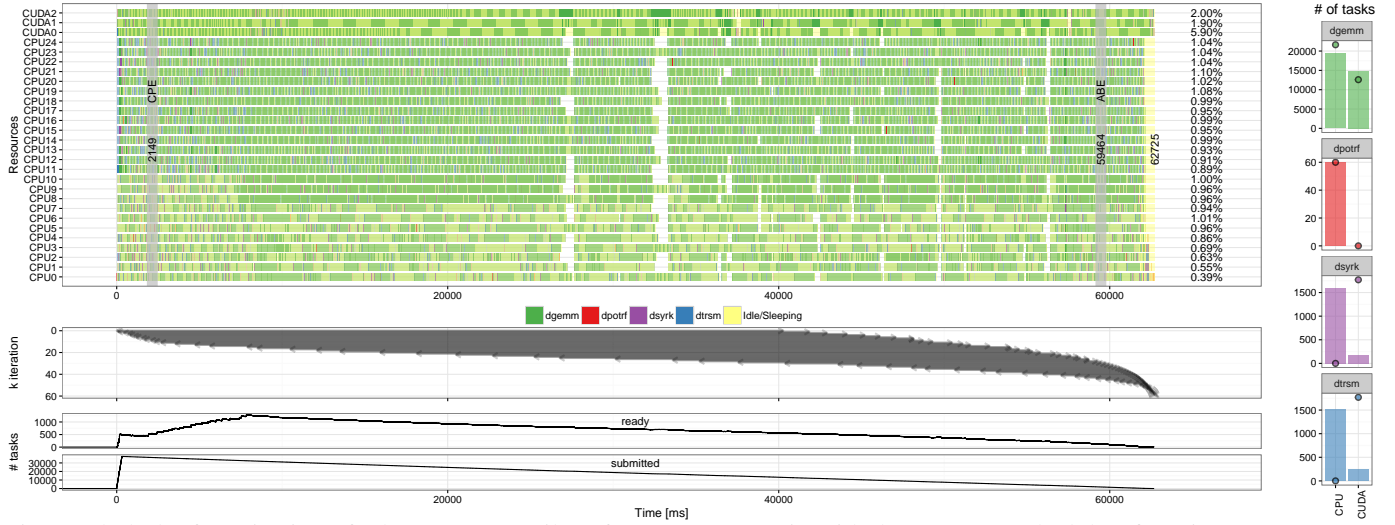
Fig. 3: Cholesky factorization of a large ( 60 \times 60 tiles of 960 \times 960 ) matrix with the DMDAS scheduler; five views are referred as indicated on the right. (a) This Gantt chart is automatically augmented with (from left to right), the critical path bound (CPE) and of the area bound estimations (ABE) and the makespan. The time percentage in the Idle state per resource is shown on the right. Finally, tasks whose duration is abnormally large compared to the others are highlighted with a darker color. (b) The plot is composed of horizontal segments, one per iteration k of the outer loop, indicating during which time interval the tasks of the iteration have been processed. (c) depicts how many tasks are finished waiting for dependencies, and thus ready for execution and (d) how many are submitted and still not executed. (e) compares the actual number of tasks of each type executed on CPUs and GPUs (the bar) with the optimal repartition obtained when computing the ABE (the bullet).
