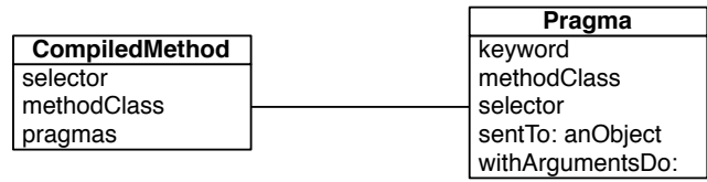
Figure 1. Pragma API.
