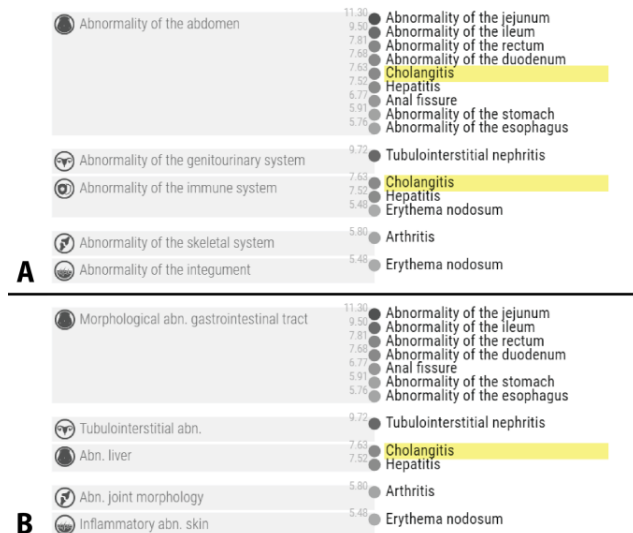
Fig. 9. Comparison between category and cluster layouts. Cholangitis, an inflammation of the liver, (A) appears under both Immune System and Abdomen in the category view, where it is grouped with mostly gastrointestinal abnormalities. (B) The cluster layout selects a more meaningful organization that separates Gastrointestinal abnormalities and Liver abnormalities using our topology simplification algorithm.
