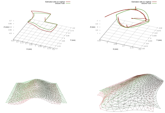
Figure 3: Results obtained on computer-generated data: [Top row] the estimated trajectory and its ground truth and [Bottom row] The recovered 3D mesh and its ground truth. (Left) elasticity = 25%, Mean error = 2.11 mm, RMS error = 2.33 mm — (Right) elasticity = 130%, Mean error = 0.96 mm, RMS error = 1.25 mm
