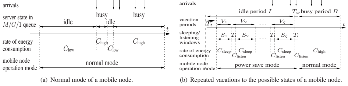
Figure 2: Mapping the M/G/1 queue .
